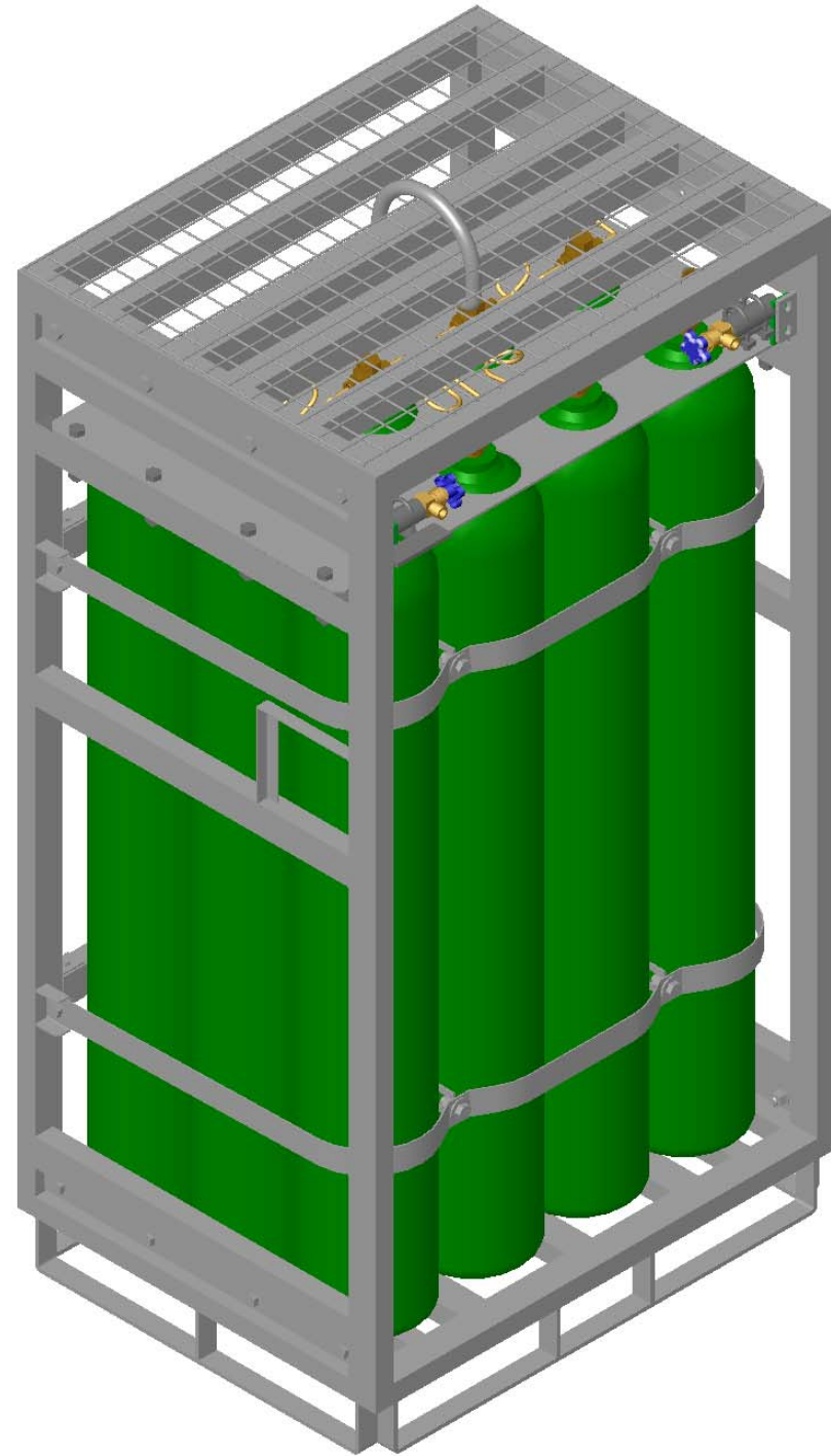
HP12PACK DC-MANIFOLD(795x1018x2000H)
